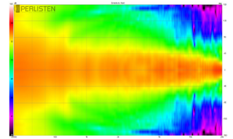
Vertical Directivity
