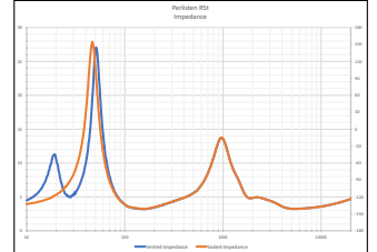
Impedance
